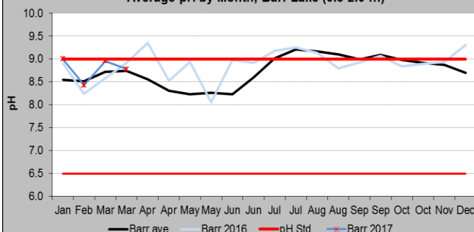
Average pH by Month, Barr Lake (0.5-2.0 m)
