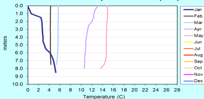
Milton Reservoir Temperature Profiles (2017)
