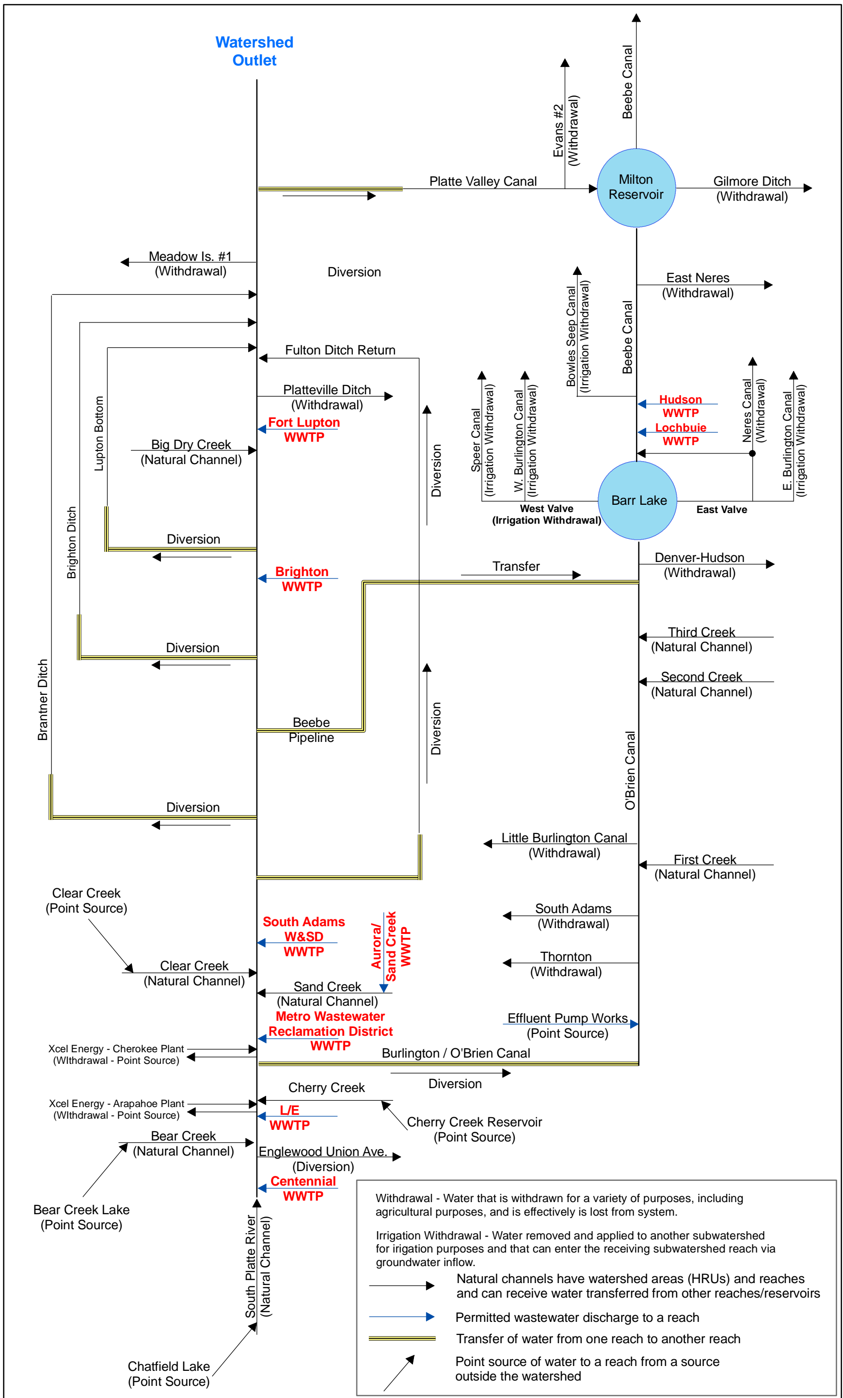
Schematic Diagram of Water Flow and Transfer within Barr-Milton Watershed For use in Setup of SWAT2005 Watershed Model
